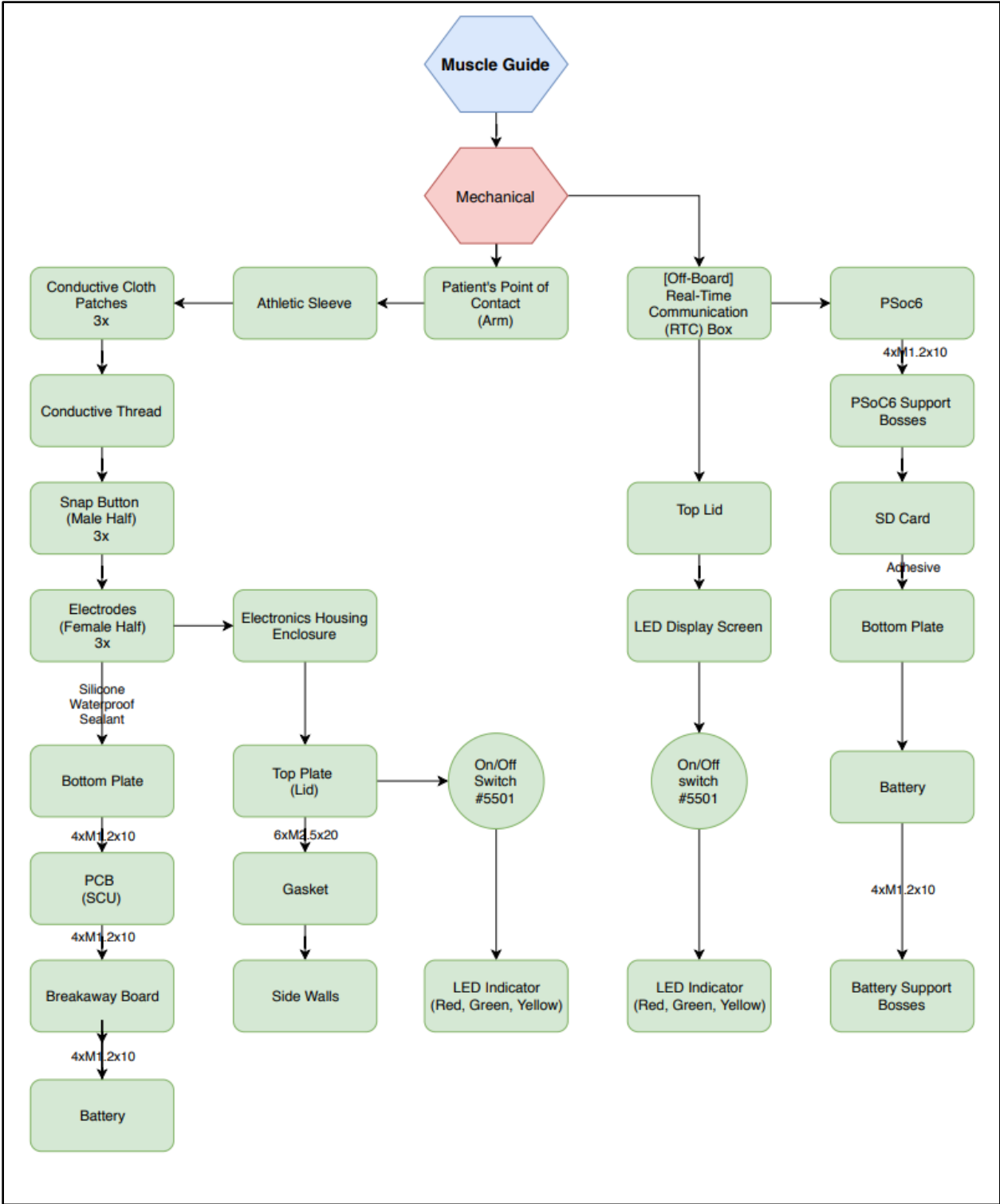
Mechanical Block Diagram 2
